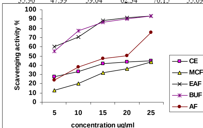
Figure (4) Scavenging activity of strawberry shoots on DPPH
