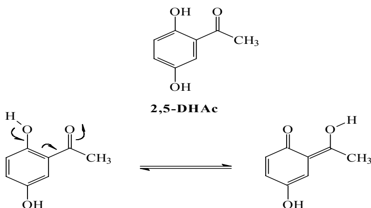
Fig. 3: The proposed mechanism of the hydrogen transfer along the structure of 2,5-DHAc showing the tautomerism between the carbonyl group and the hydroxyl group
